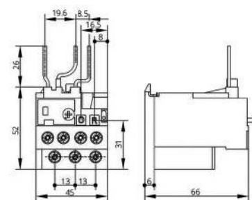
Relè BR30
