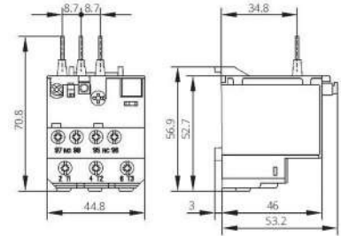
Relè BR6
