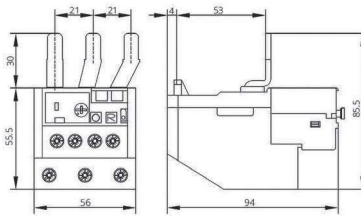
Relè BR63
