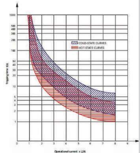
BR63
